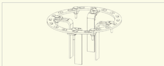
PIX04-2 Circular bracket for assembling your 3D decorations Inner diameter adjustable
