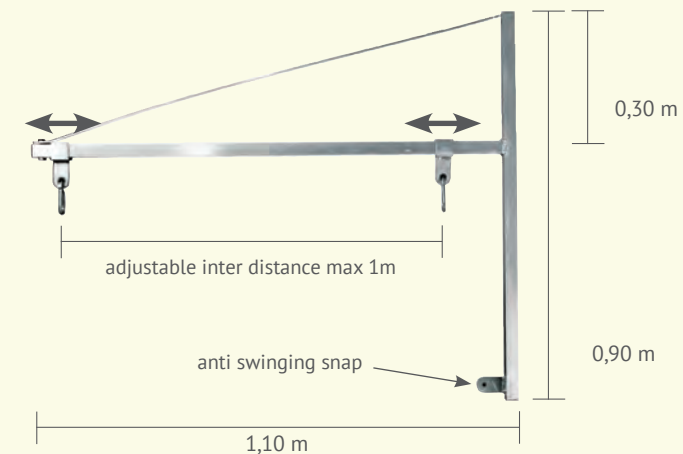
PIX01 Horizontal bracket H: 0,90 m - L: 1,10 m Inter distance max: 1,00 m Load max: 25 kg
