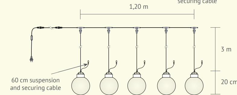
60 cm suspension and securing cable
